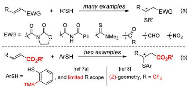
Scheme 1. Reported Catalytic Asymmetric Sulfa-Michael Addition
