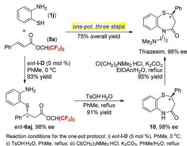
Scheme 2. Concise Synthesis of ( R )-Thiazesim
